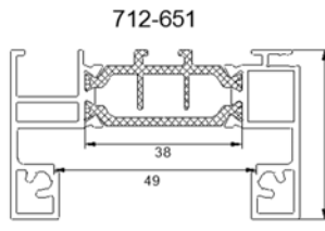
traverses basses
