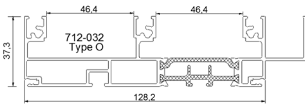
traverses basses
