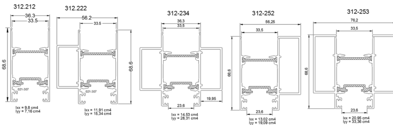
Montants 28 mm
