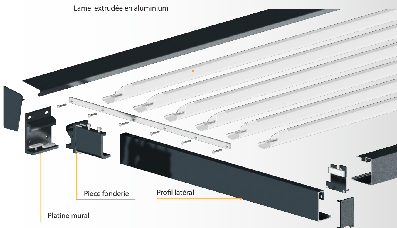
Lame BSO MATHILDA PBSO63
